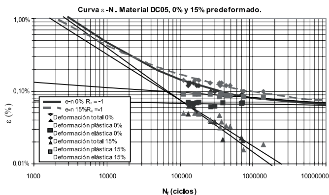
Figura 3. Curvas \epsilon -N de Material DC05.
